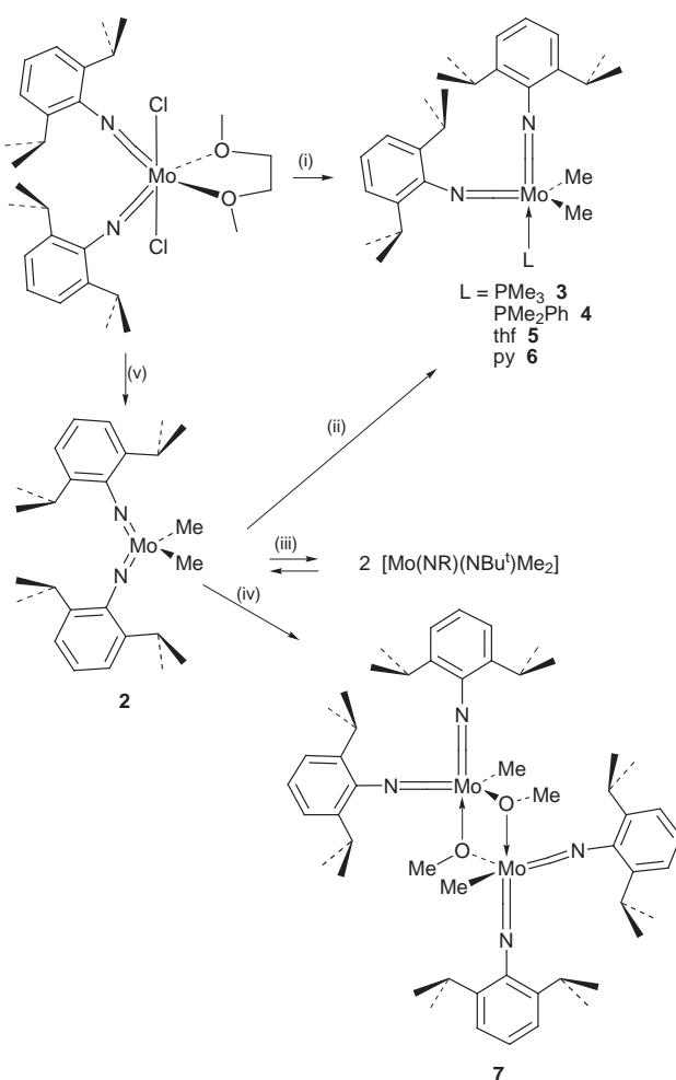
Scheme 1 (i) \text{PR}_3 , 2\text{MgMeBr} , \text{Et}_2\text{O} ; (ii) thf or py, room temperature (r.t.); (iii) [\{\text{Mo}(\text{NBU}^t)_2\text{Me}_2\}]_2 , benzene, r.t.; (iv) \text{O}_2 , toluene, r.t.; (v) 2\text{MgMeBr} , \text{Et}_2\text{O} .
